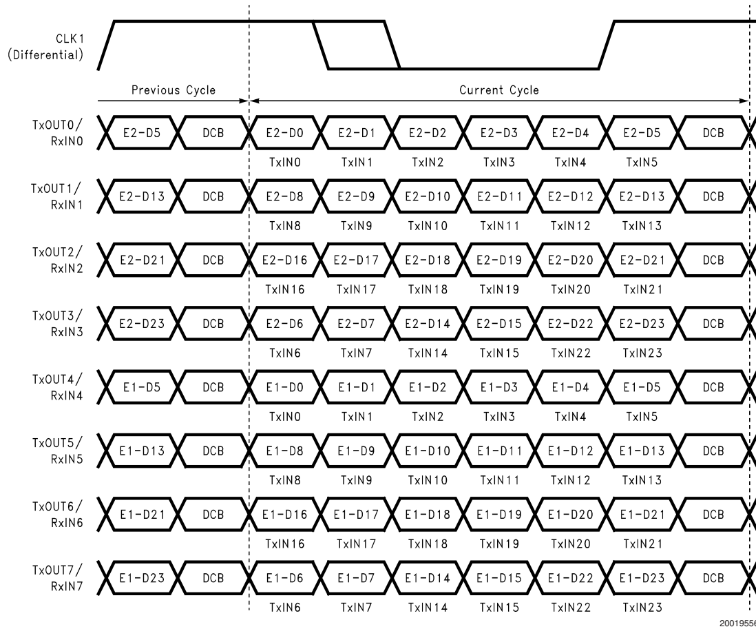
FIGURE 10. 48 LVTTL Inputs Mapped to 8 LVDS Outputs (DC Balance Mode- Enabled; BAL = High) (E1 - Falling Edge; E2 - Rising Edge)
