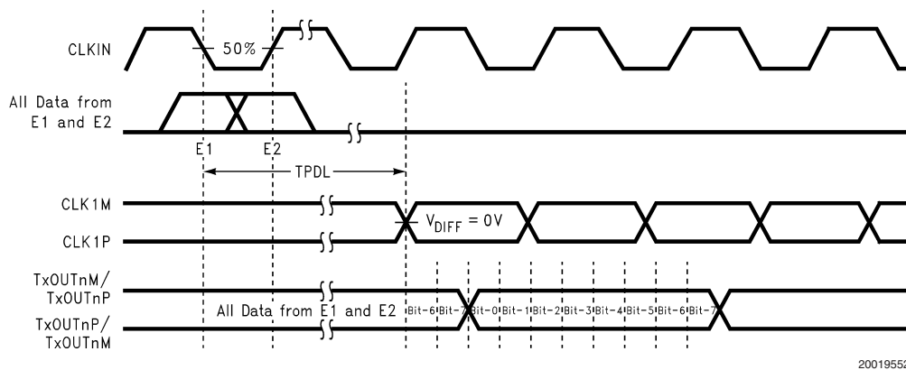
FIGURE 8. Input to Output Latency
